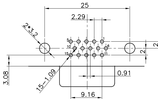
PCB Holes Diagram Top View
