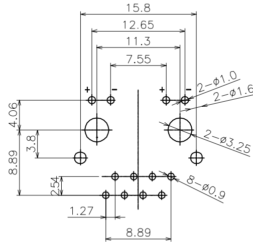
PCB LAYOUT (BOTTOM VIEW) RECOMMENDED
